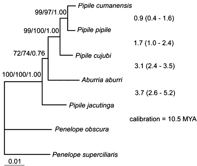
Fig. 2. Bayesian tree topology obtained from the combined analysis of CR, cyt b , and ND2 sequences. Bootstrap values obtained for MP and ML and posterior probabilities from BA for each node are indicated to the left of the tree. Estimates of divergence times (confidence intervals) based on a penalized likelihood approach are also shown to the far right of each node.
