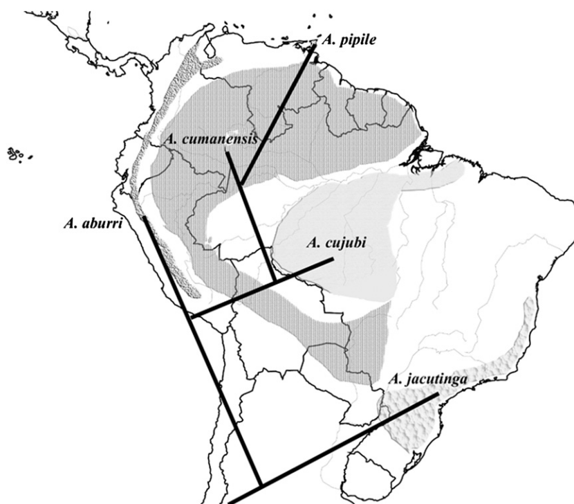
Fig. 1. Phylogeographic distribution of Aburria spp. Modified from Delacour and Amadon (1973) and phylogenetic relationships as estimated in the present study based on mitochondrial DNA sequences.
